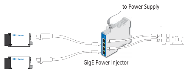
Improved GigE Power Injector configuration
